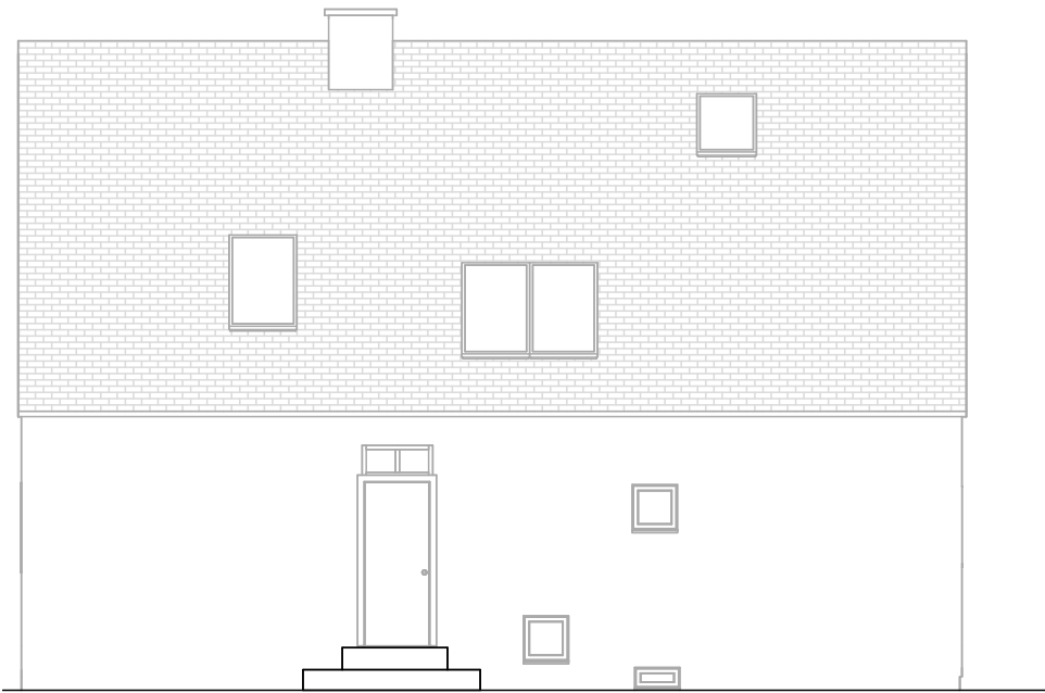
4 WEST ELEVATION 1 : 100
